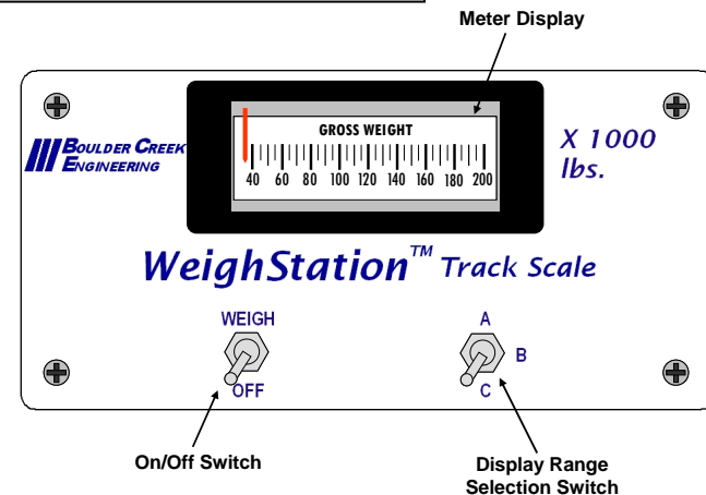
Figure 2: Faceplate Controls
